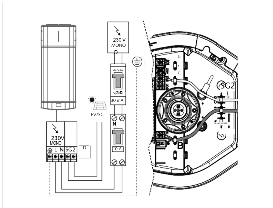
Fig.: PV o SMART GRID (SG2)
