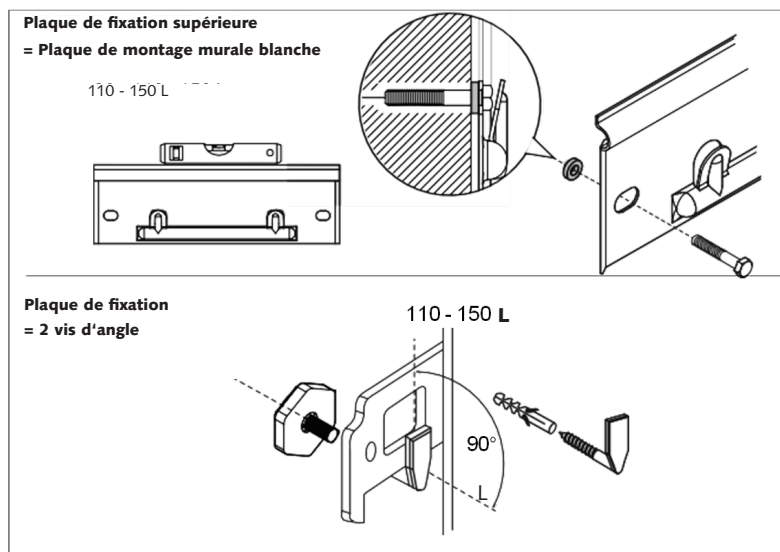
III. : Montage mural
