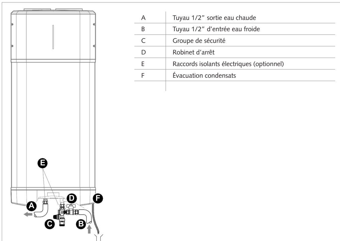
III. : Raccords hydrauliques
